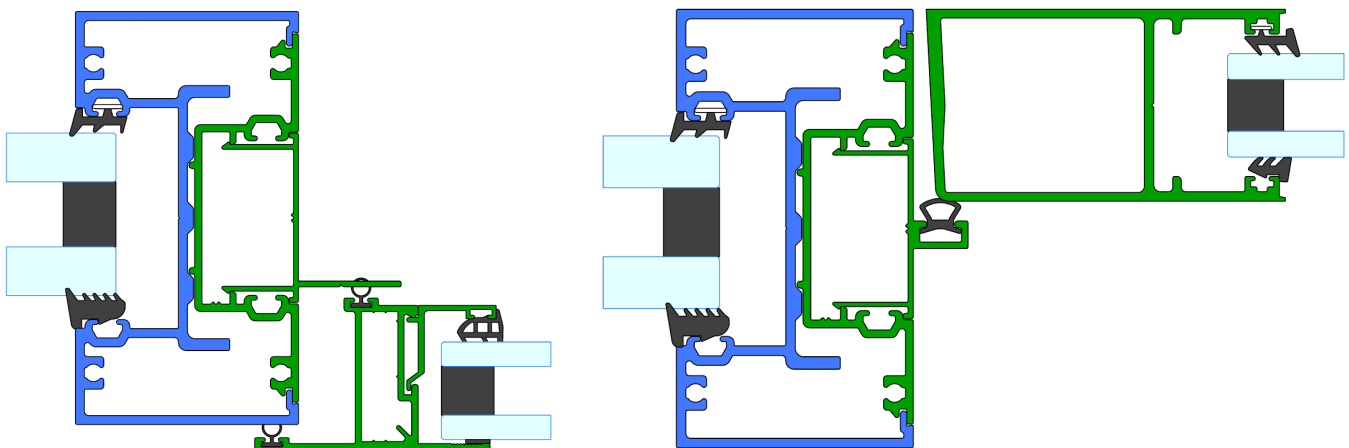
50mm Pocket sections (blue) coupling with awning and hinge doors (green)
