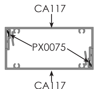
Blind Split Mullion
