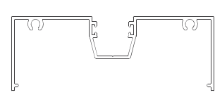
OP163 Mullion/Transom
