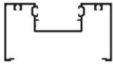
Frame 100mm x 55mm DF400 6500mm
