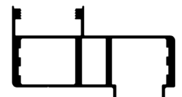
3 Panel Adapter
