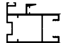
S/G Interlock
