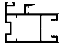
S/G Interlock
