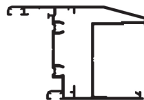
Sash Double Glazed
