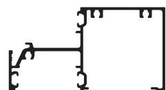
Externally Glazed Sill/Transom FDG512 Length: 6500
