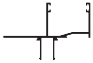
S/G head/Sill Adapter DHW111 Length: 6500 To suit CA460
