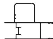
D/G Female Stile DGS82 Length: 6500
