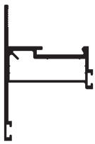
Flat Awning Sash CA470 Length: 6500
