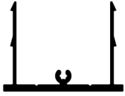
50mm Batten Base BTB 6500mm To suit BT50/ BT100/BT150/ BT200/BT300
