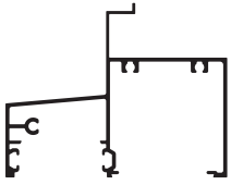
Inline Sash Sill FDG519 Length: 6500
