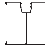
76mm Corner Post CA308 Length: 6500
