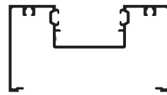
Frame DF400 Length: 6500
