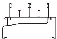
Sill / Transom DF416 Length: 6500
