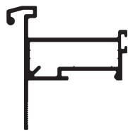
Flat Sash w/Hinge CA471 Length: 6500
