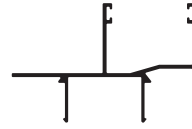
10044-DG Head/Sill Adapter DHW116 Length: 6500 To suit CA500
