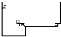
100mm Gutter Sill GS1 Length: 6500 To suit 101mm frames
