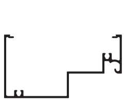
Inline Sash Transom/Head DF411 Length: 6500
