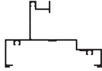
Head/Sill ULT-F26 Length: 6500
