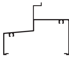
Inline Sash Transom/Sill DF412 Length: 6500
