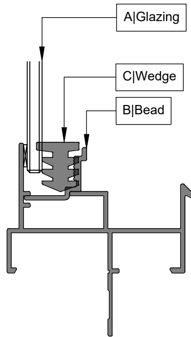
CSW3 Sill CSW12 Bead
