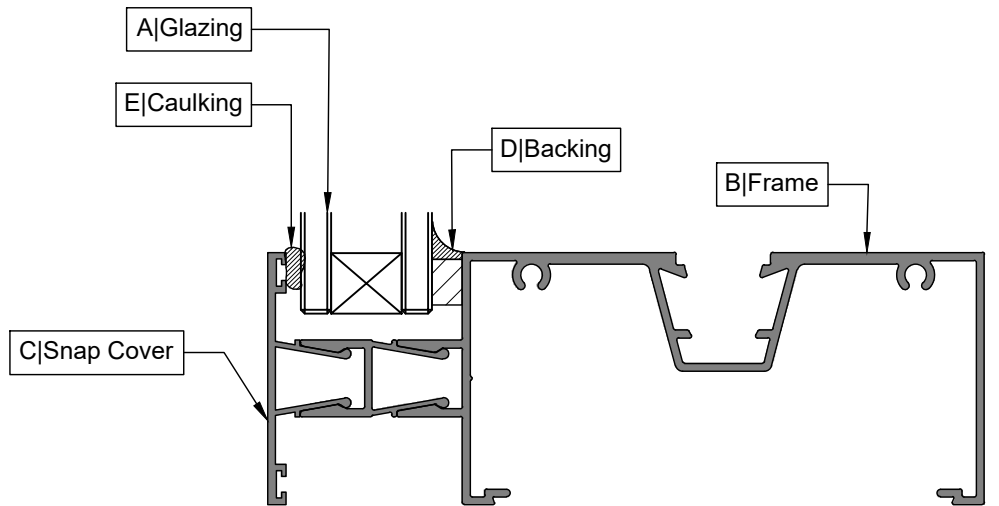
CA111 S/G Frame with CA809 Adapter CA810 Snap Cover
