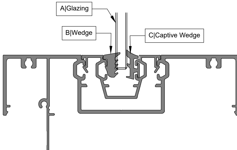
DJ125 Frame DF606 SG Pocket Reducer
