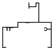
Head/Sill ULT-F400 Length: 6500
