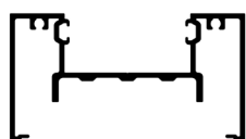
Frame DF450 Length: 6500
