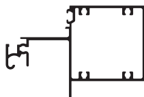
Beaded Inline Sash Transom FDG517 Length: 6500
