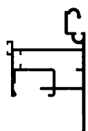
Inline Hook Sash FDG522 Length: 6500
