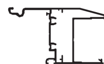
Hook Sash Double Glazed F63 Length: 6000
