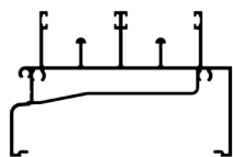
Sill / Transom DF416 Length: 6500
