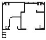
Head BF1 Length: 4500/6500
