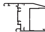
Sash Double Glazed F62 Length: 6000
