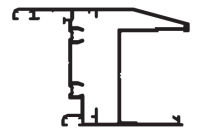
Sash Double Glazed F62 Length: 6000
