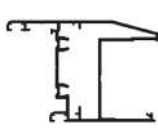
Sash Double Glazed F62 Length: 6000
